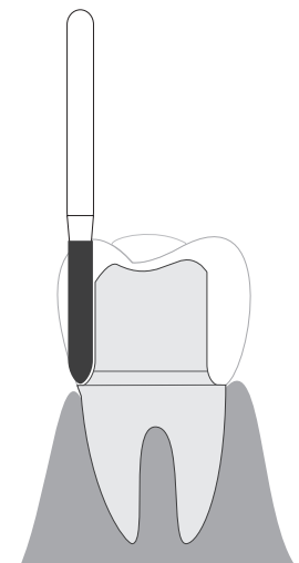
878 Cylindrical Torpedo Modified chamfer preparation.
